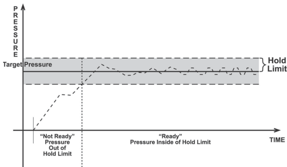
Figure 5. Ready/Not Ready in Dynamic Pressure Control Mode
