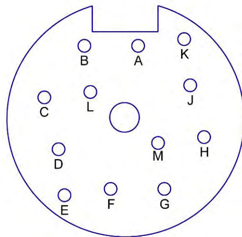
Figure 19. Drivers Connector Schematic
