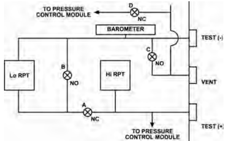
Figure 18. PPC4E Reference Pressure Transducer Module Schematics
