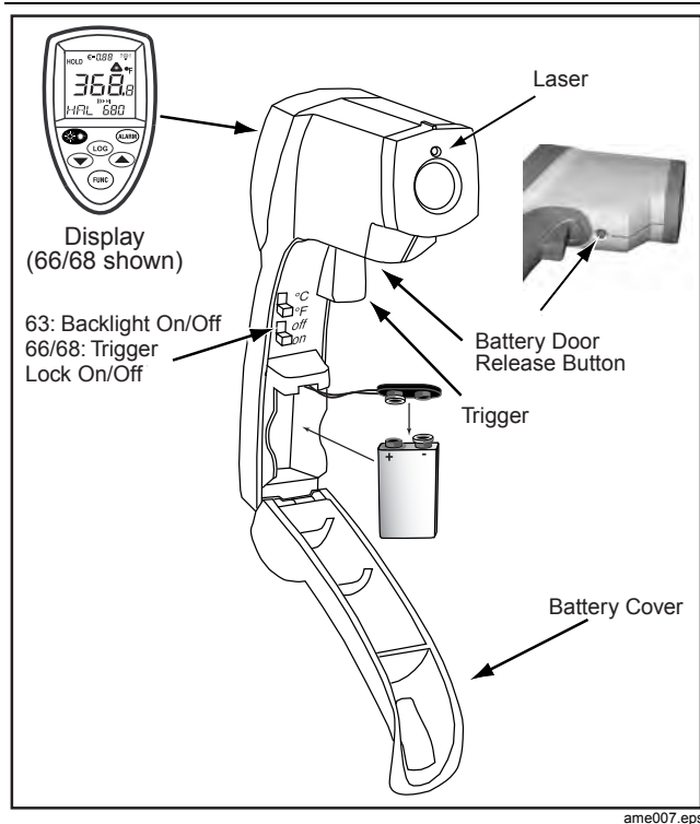
Figure 2. Infrared Thermometer
