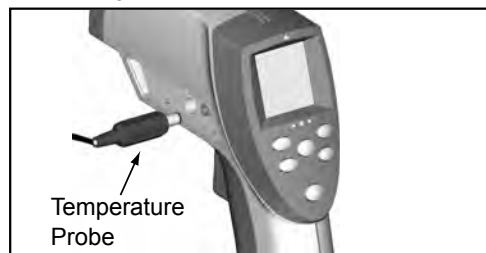
Figure 8. Connecting a Temperature Probe
