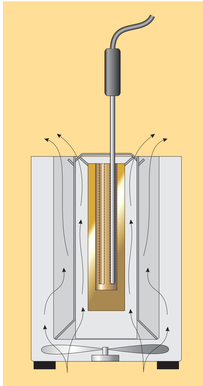
Simplified schematic illustrating the airflow design (patents applied for) to minimize potential heat damage to sensor handles and transition junctions.
