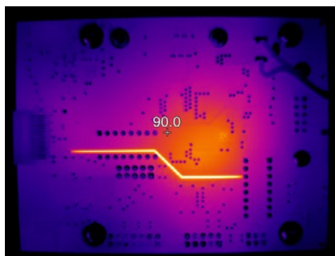
Circuit board
